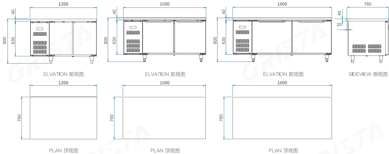
Three Views 三视图
